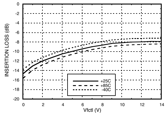
Insertion Loss vs. Temperature, Vfctl = Vbwctl
